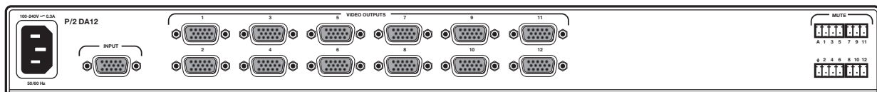
P/2 DA12 - Back
